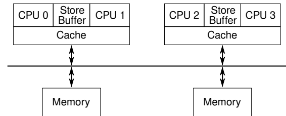
Figure 15.13: Shared Store Buffers And Multi-Copy Atomicity
