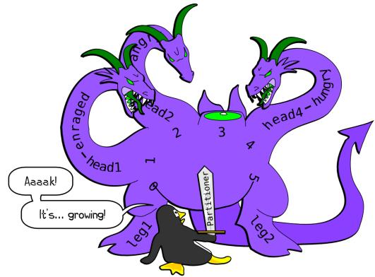
Figure 10.13: Partitioning Problems
