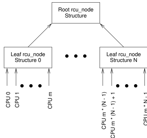
Figure 7.10: Locking Hierarchy
