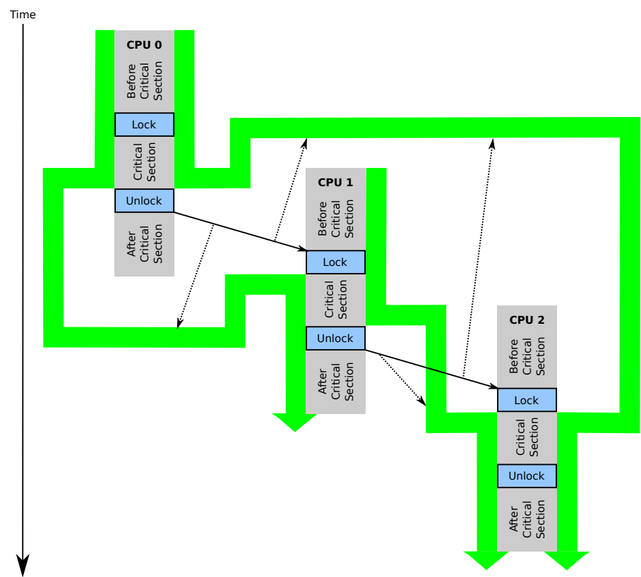
Figure 15.1: Locking Intuitions
