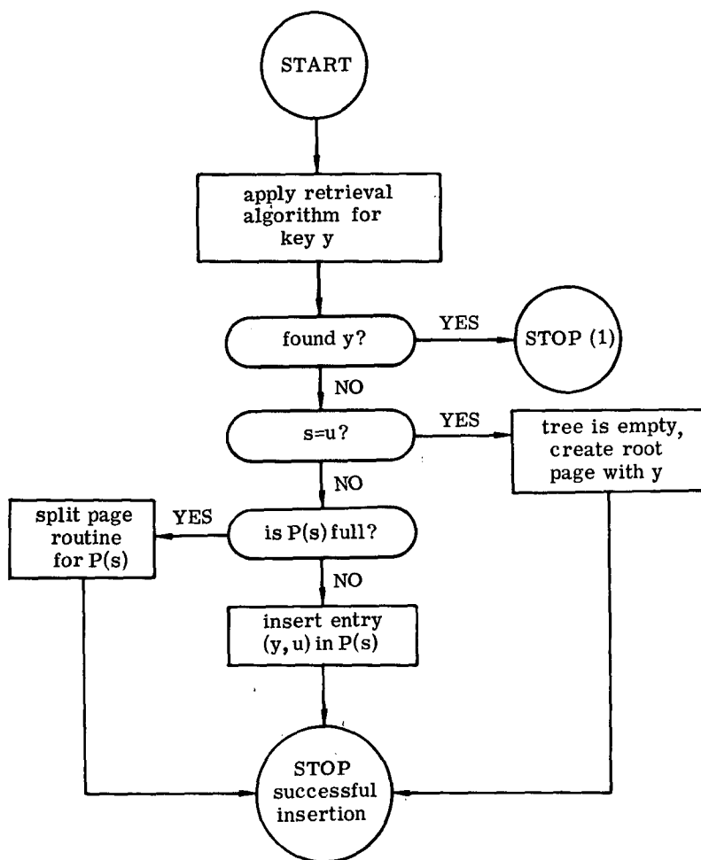
Figure 4. Insertion Algorithm
